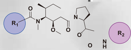
Auristatin
